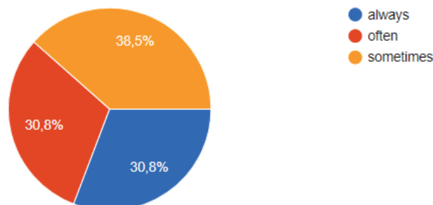
Graph 4 Learners' answers
